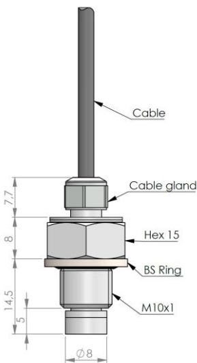
LOW LEVEL IP67 CABLE OUTPUT
