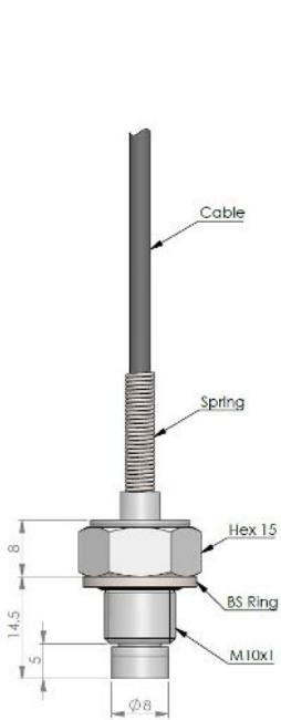
LOW LEVEL CABLE OUTPUT
